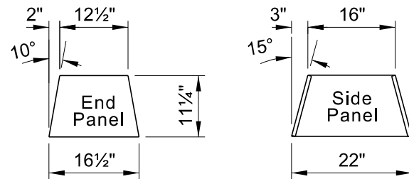
#5 Wood Form 12" x 14" Frame and Cover
