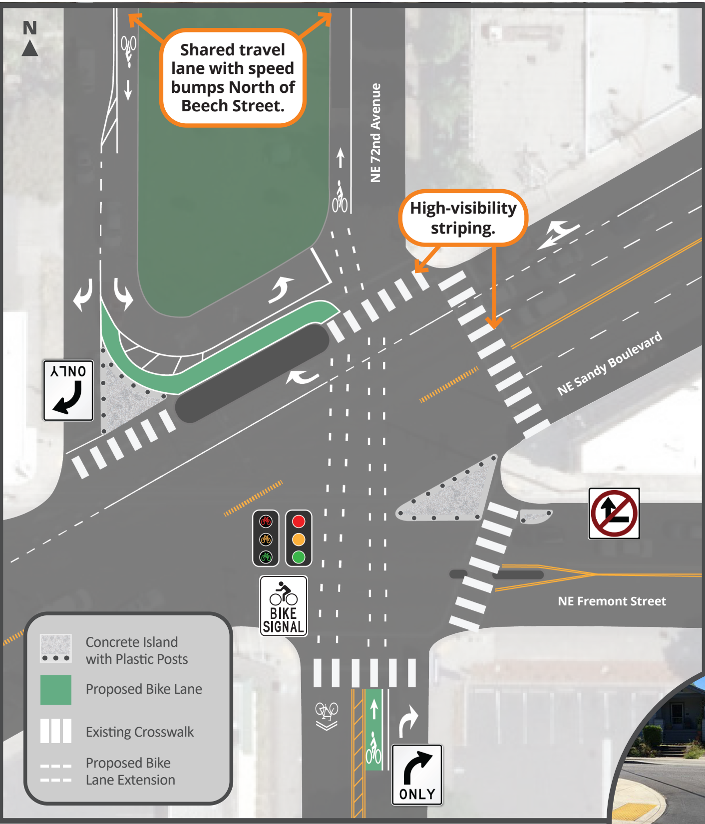
NE 72nd Avenue: Sandy Boulevard and Fremont Street INTERSECTION IMPROVEMENTS: 60% DESIGN PLANS
