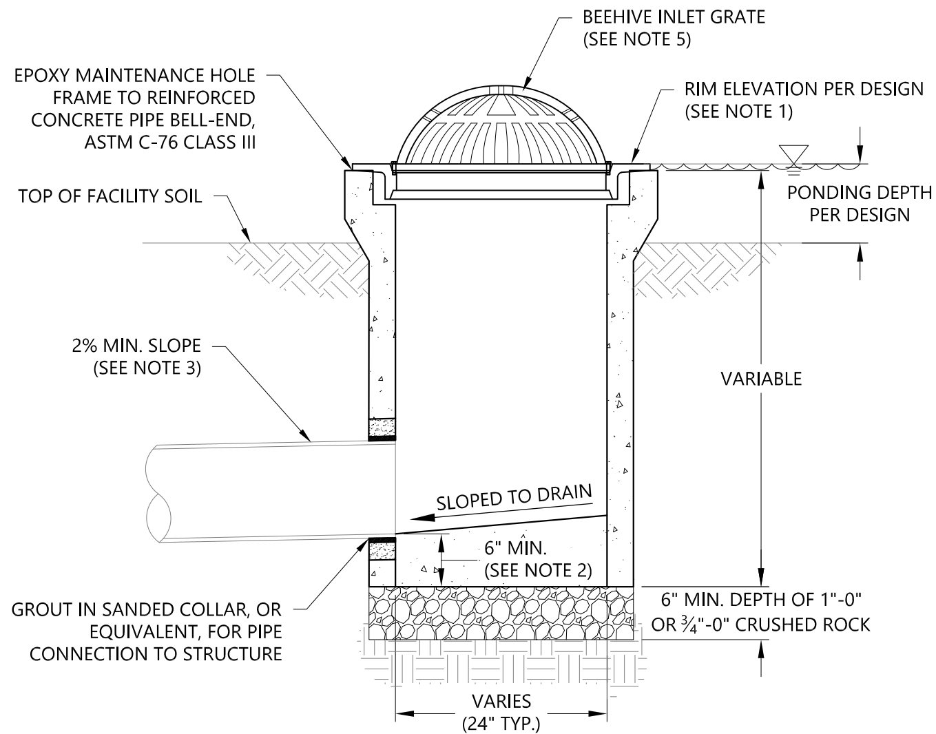
BEEHIVE INLET - SECTION
