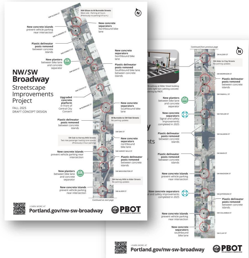
Draft concept designs. Images by PBOT.
