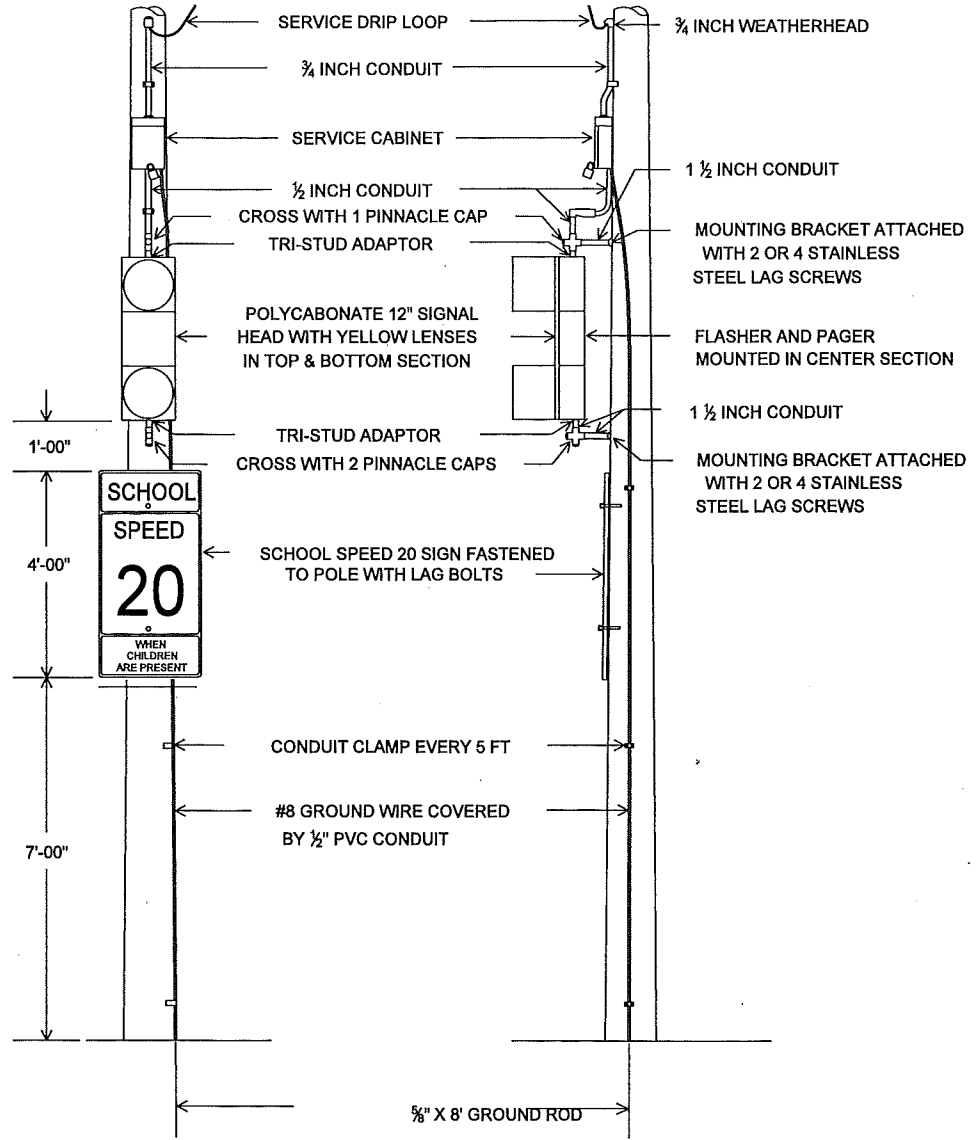
"SCHOOL ZONE FLASHER" SIGNAL & ILLUMINATED SIGN MOUNTING ON WOOD POLE
