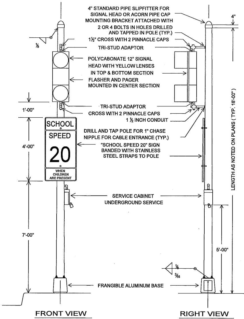
"SCHOOL ZONE FLASHER" SIGNAL OR ILLUMINATED SIGN MOUNTING ON FRANGIBLE BASE
