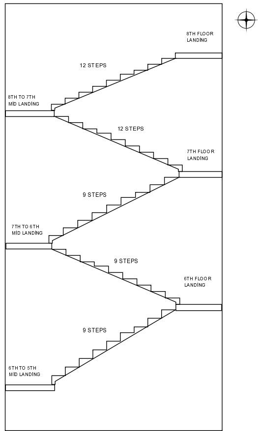
CROSS SECTION OF STAIRWAY #1 (EXHIBIT 1)
